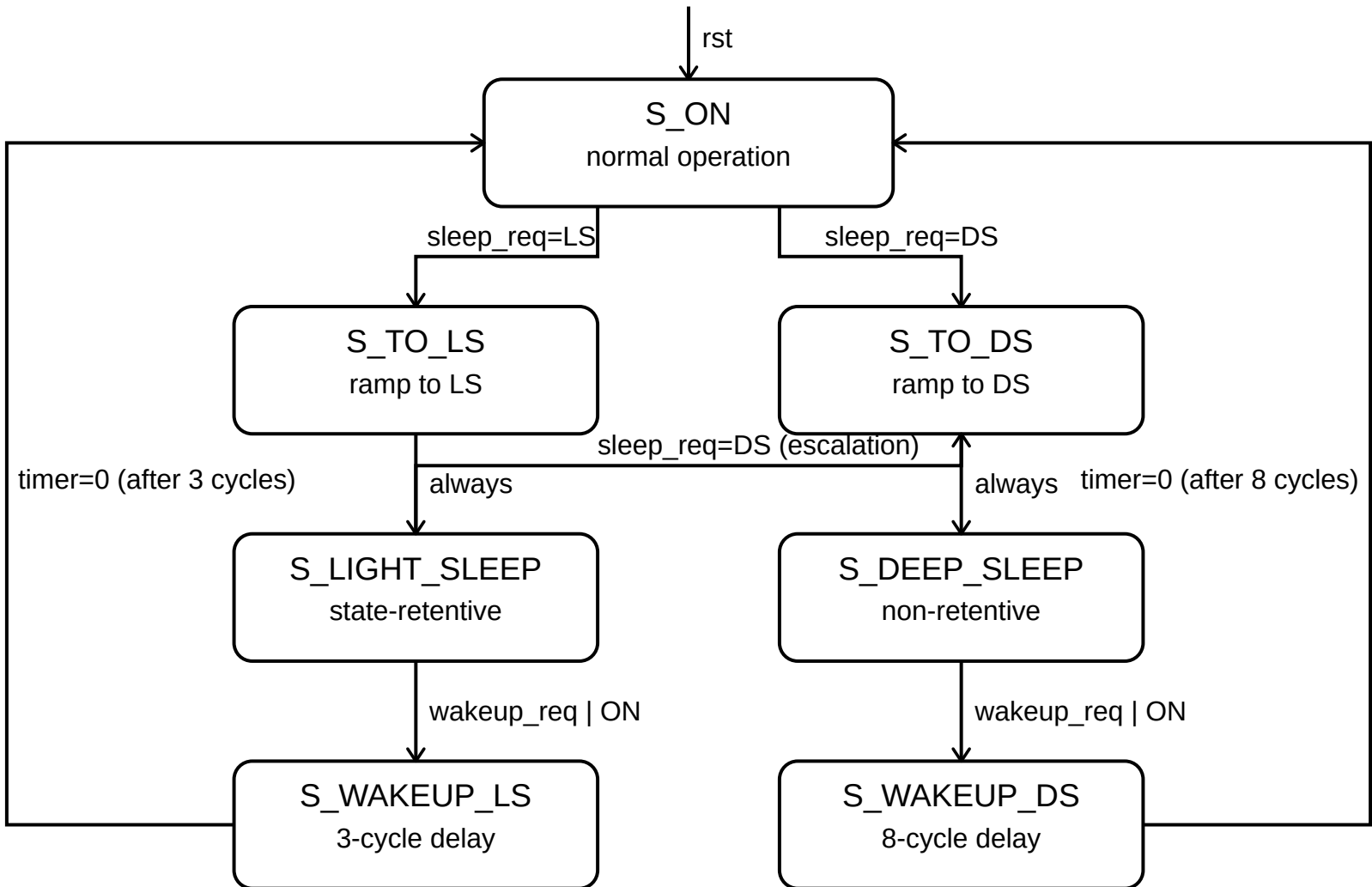
Diagram 2 — Power State FSM (7 states)
